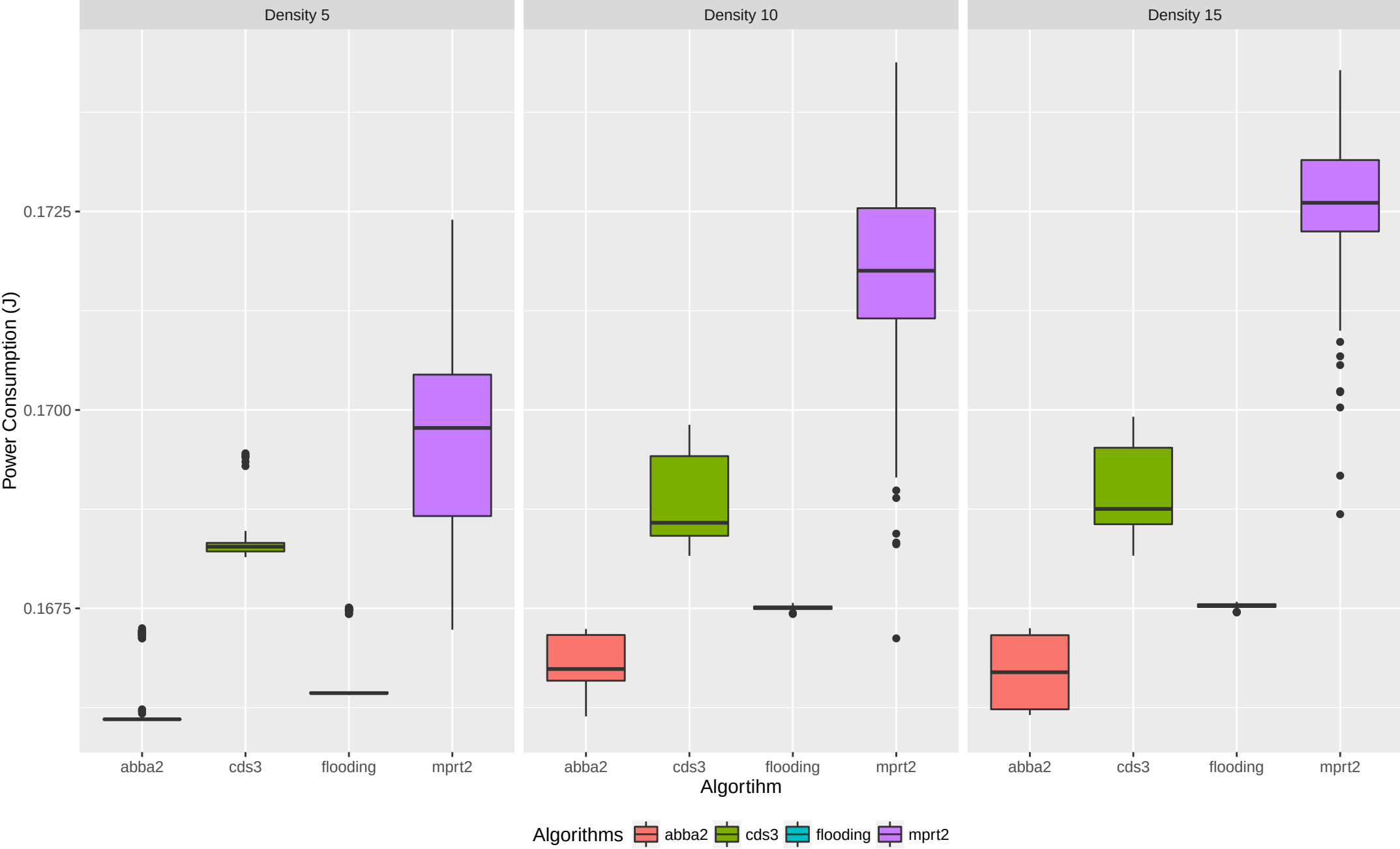
Power consumption for different algorithms
